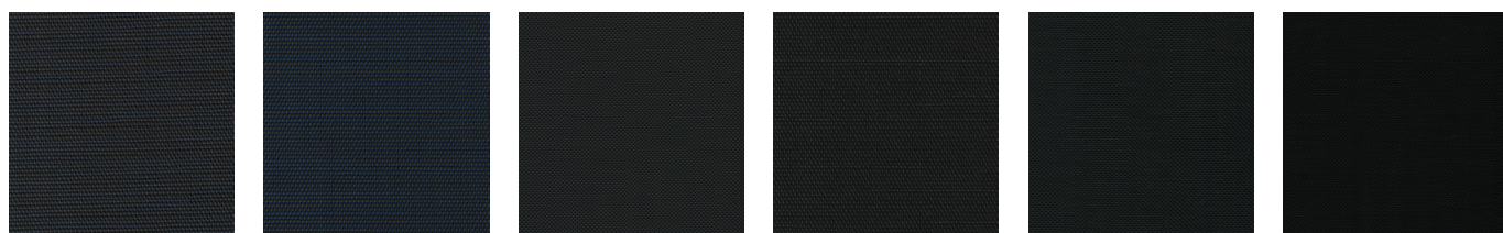
50963 SOLTIS TOUCH 5% g_{TOT} 0.51 | 50944 SOLTIS TOUCH 5% g_{TOT} 0.51 | 001 SCREEN 767 g_{TOT} 0.53 | 50940 SOLTIS TOUCH 5% g_{TOT} 0.51 | 010 MESH g_{TOT} 0.55 | 010 SCREEN 767 g_{TOT} 0.55
